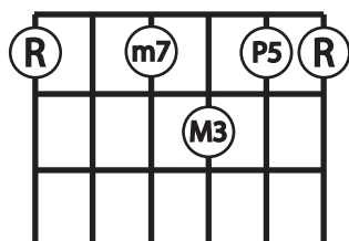
Dominant 7th
