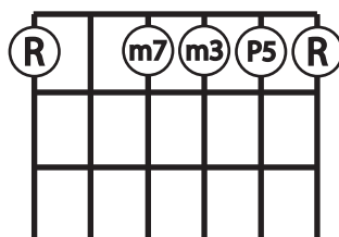
Minor 7th
