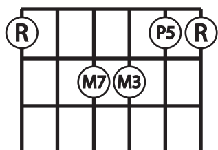
Major 7th
